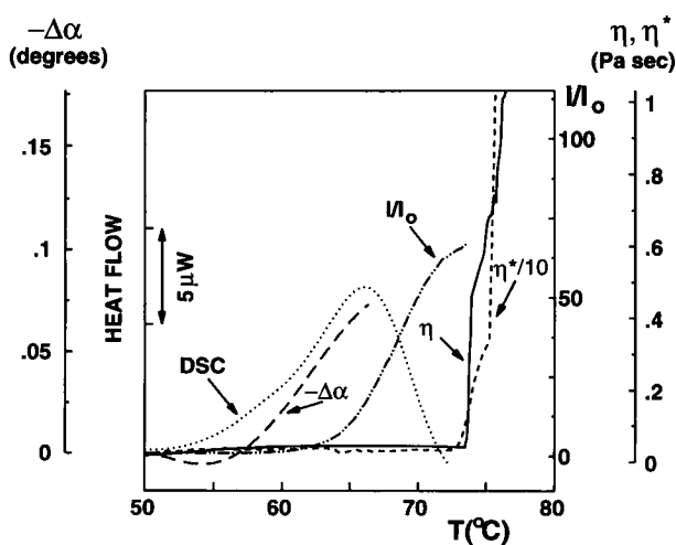
FIGURE 1 DSC, optical rotation ( \Delta\alpha ), scattered light intensity ( I/I_0 ), low-shear viscosity ( \eta ), and complex viscosity ( \eta^* = (\eta'^2 + \eta''^2)^{1/2} ) relative to a 1% w/v ( \Phi = 0.73\% v/v) solution of native BSA, measured in the course of heating at a rate of 0.05°C/min. Note that the DSC curve is attributed to protein unfolding so that the accompanying \Delta\alpha signal also monitors unfolding, whereas processes monitored by the I/I_0 , \eta , and \eta^* curves start when the specimen is a sol of already unfolded BSA.
